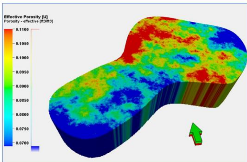
Figure (11). An effective porosity model for zone 1 of the Nubian reservoir
